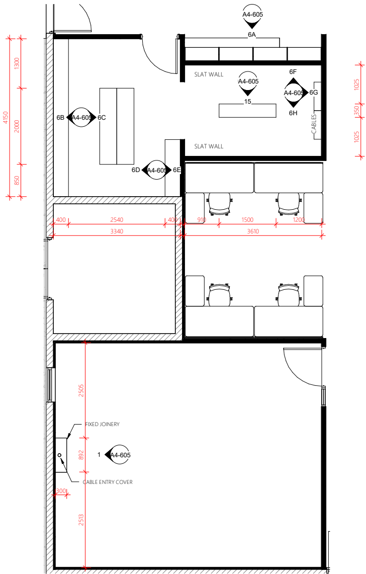
Internal Plan 2 - Consumables
