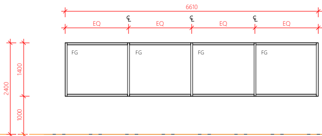
WINDOW TYPE A
