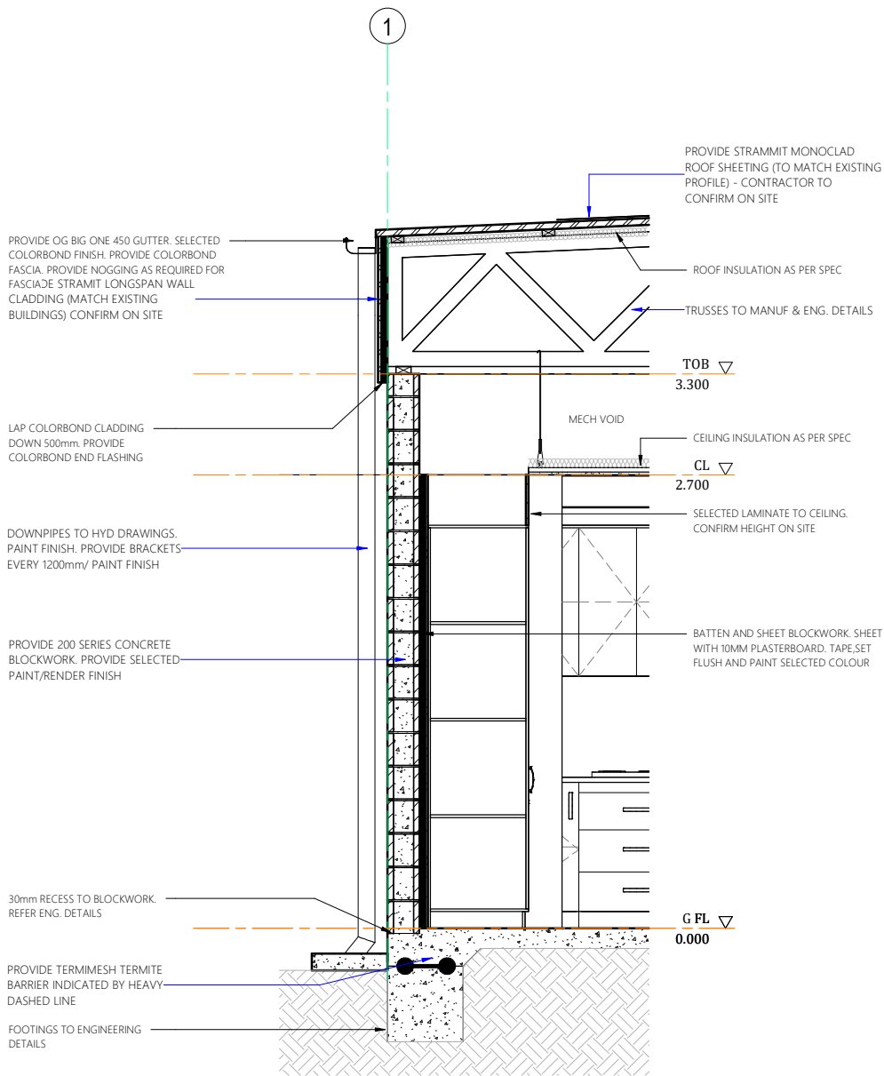
Section Detail C1
