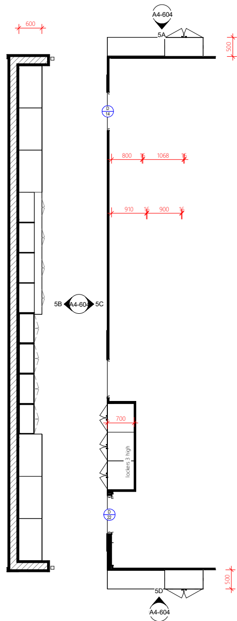
Internal Plan 5 - Central Corridor
