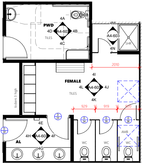
Internal Plan 3 - Amenities
