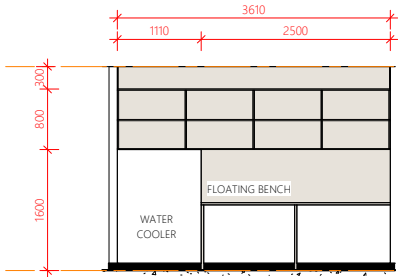
Elevation 6A
