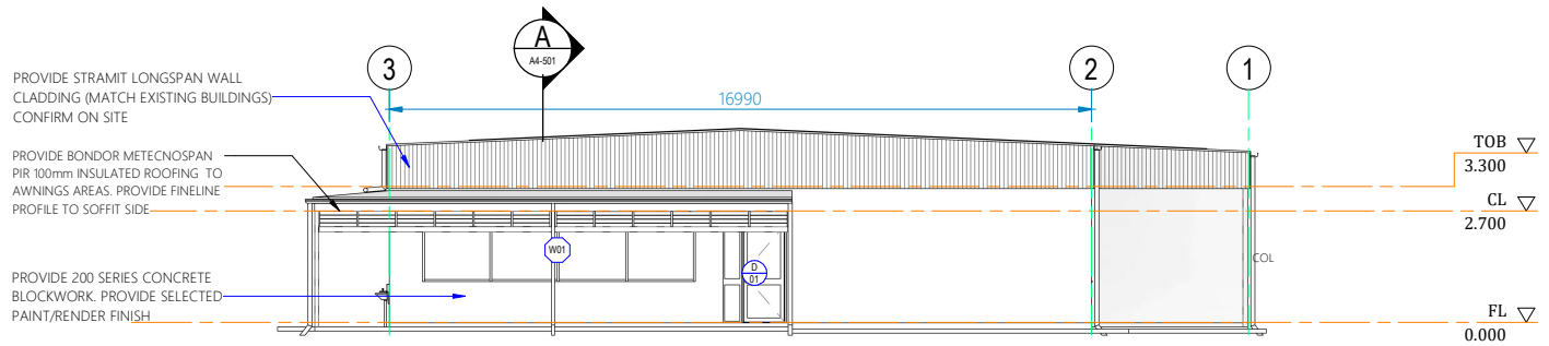
Proposed Elevation 3
