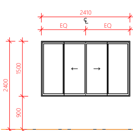
WINDOW TYPE E
