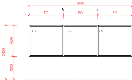
WINDOW TYPE B
