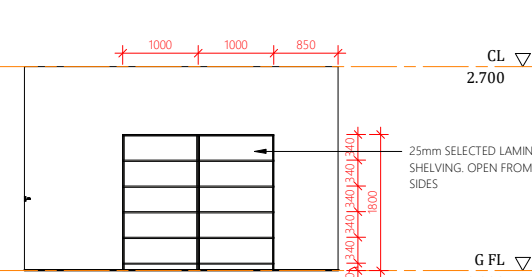
Elevation 6C
